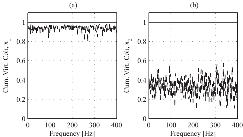
Figure 15.10 Figure from Example 1. In (a) the cumulated virtual input coherence functions g_{11}^2 (dashed) and g_{1:2}^2 for input signal x_1 . In (b) the cumulated virtual input coherence functions g_{2:1}^2 (dashed) and g_{2:2}^2 for input signal x_2 . The figure shows that the first input signal is strongly correlated with the first virtual input, whereas the second input signal is a little less correlated with, but still dominated by, the second virtual input. The less correlation in the latter case is due to the fact that x_2 is somewhat correlated with x_1
