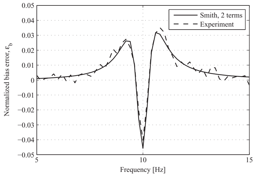
Figure 10.6 Experimental bias error calculated on a PSD using the Hanning window and Welch’s method, from simulated data of an SDOF system with an FFT frequency increment \Delta f = B_r/5 . See text for details. In the figure it is shown that the experimentally obtained normalized bias error agrees very well with the theoretical expression of the bias error given by Equation (10.20). The variations in the experimentally obtained bias are due to the random error in the estimate of G_{xx}
